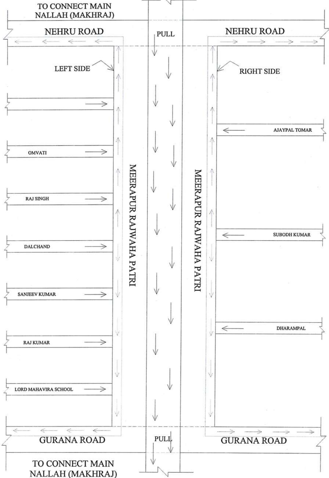
SEWAGE WATER DIVERSION SITE PLAN OF MEERAPUR RAJWAHA
